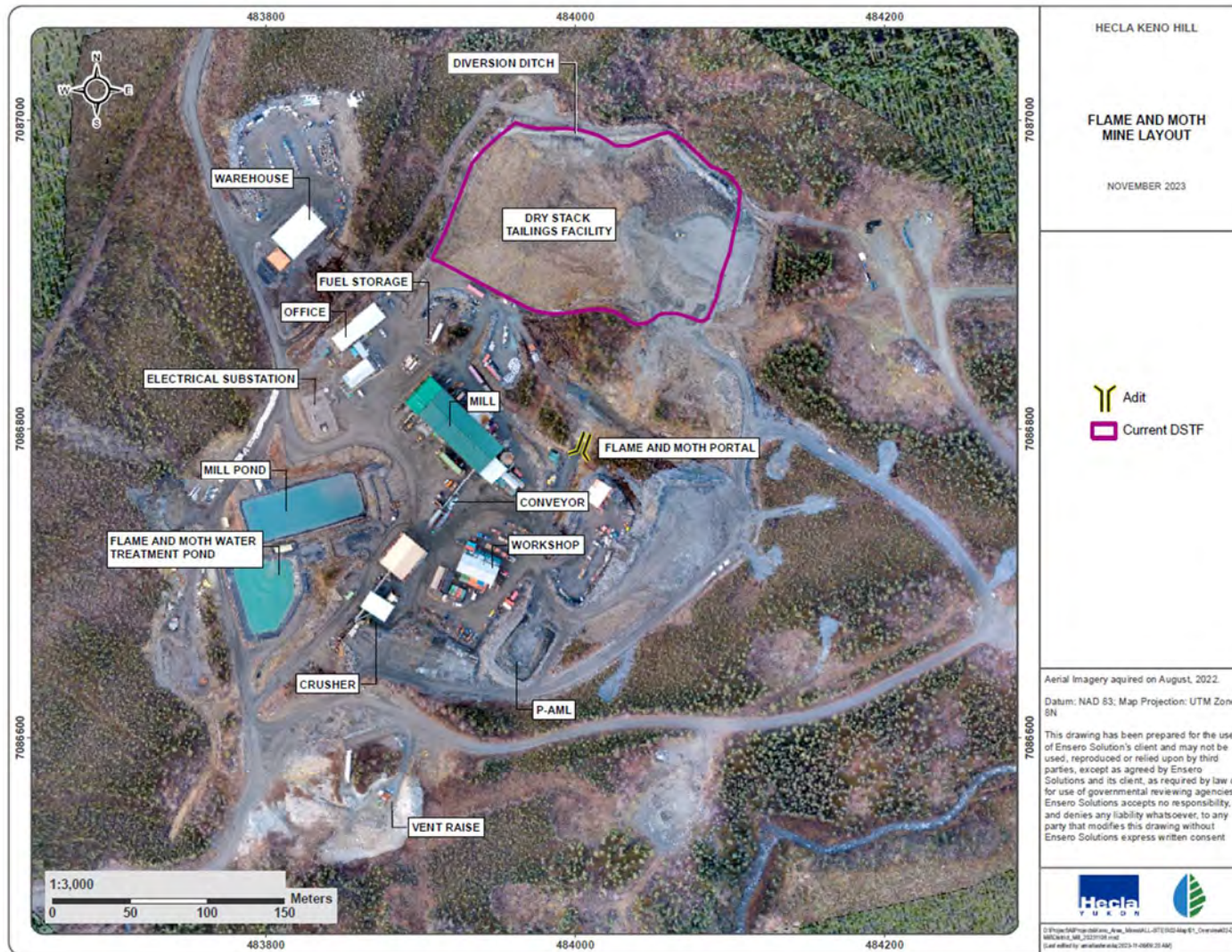
Figure 15-4 – Flame and Moth Site Layout.
