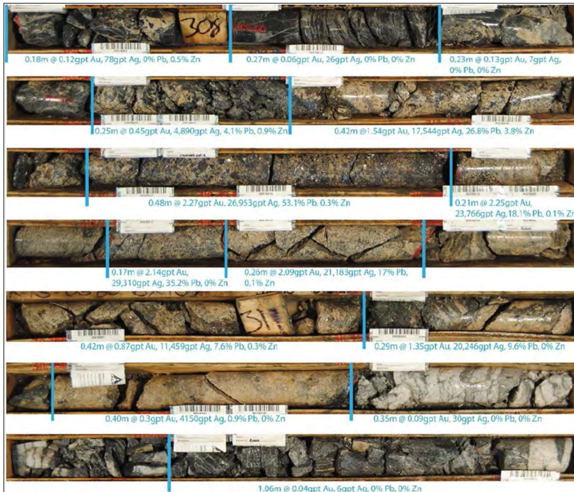
Figure 6-11 – Vein-Fault Intercept in Drill Hole K-15-0580 in the Bermingham Deposit (Mining Plus, 2019).
