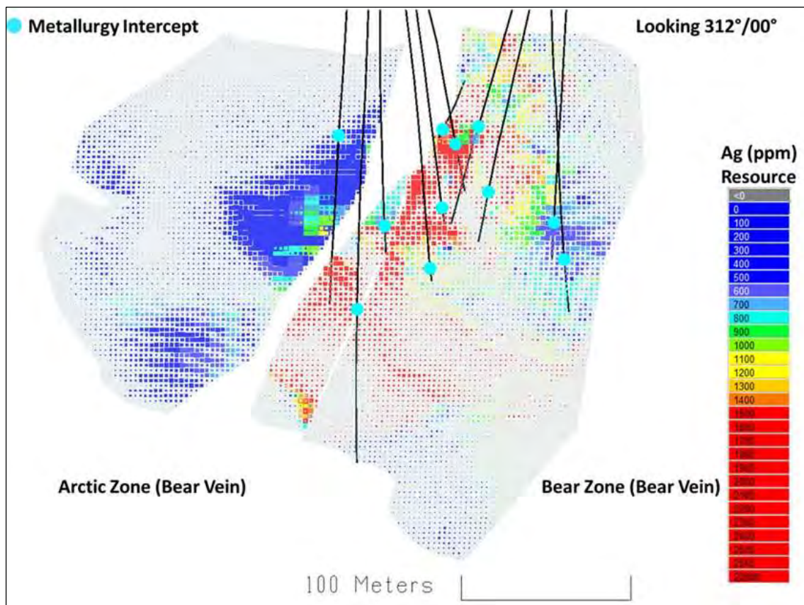
Figure 10-2 – Source of Metallurgical Samples from Birmingham (Alexco, 2021b).
