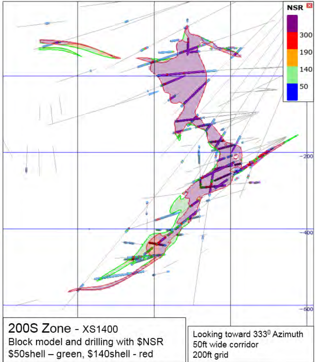
Figure 6-39: 200S Zone – Cross Section 1400
