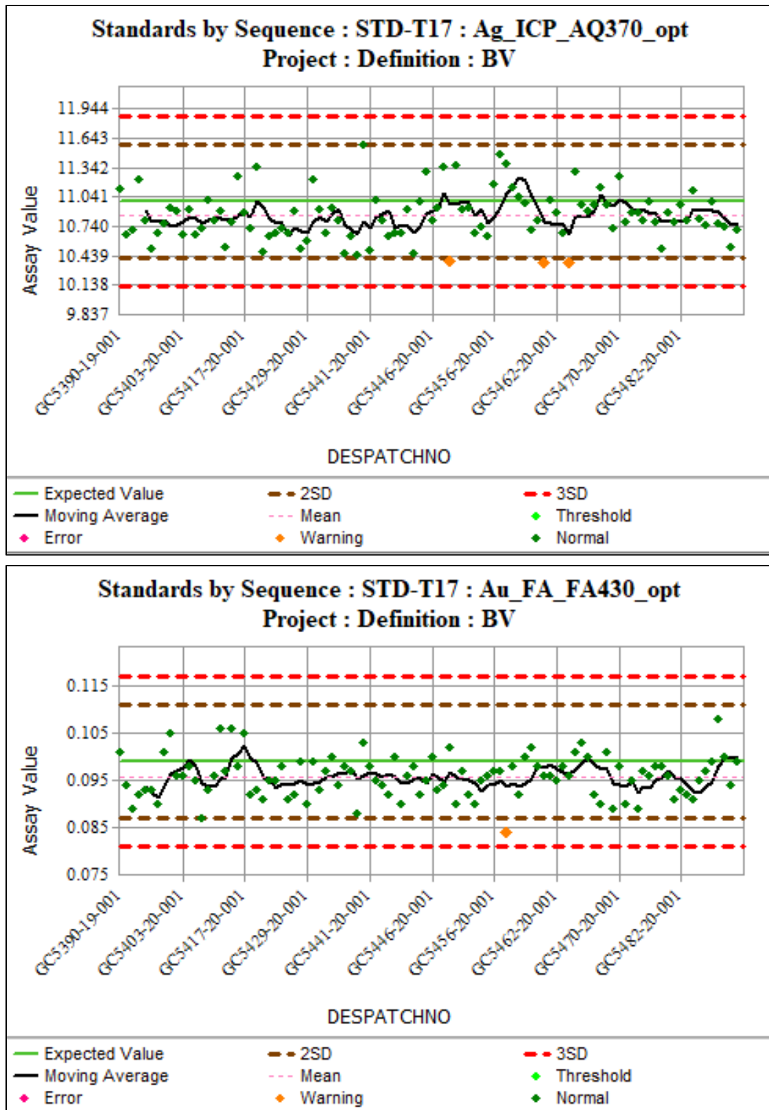
Figure 8-1: Standard Control Charts – Standard T17: Ag, Au – Bureau Veritas 2020
