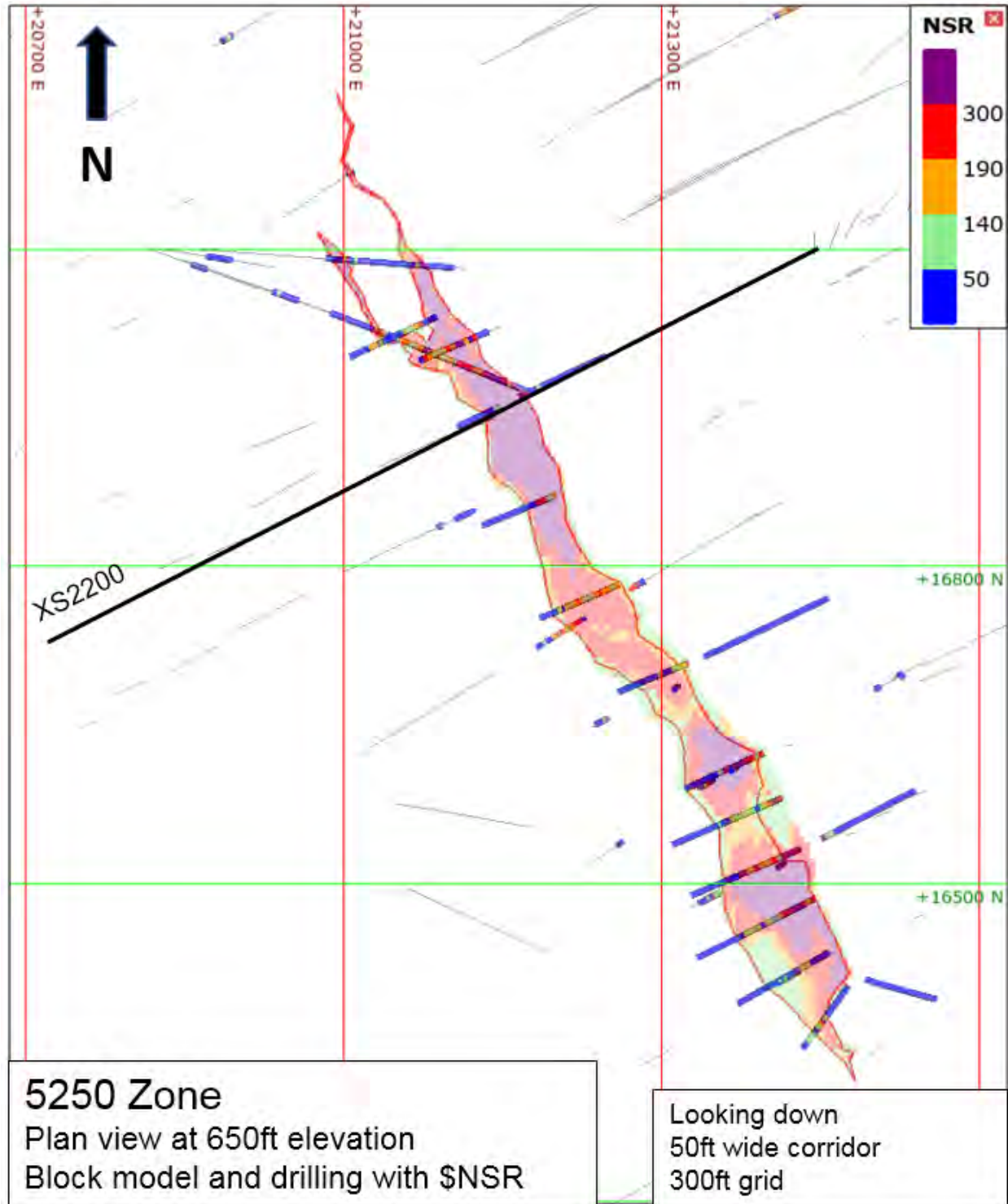
Figure 6-32: 5250 Zone – Level 650
