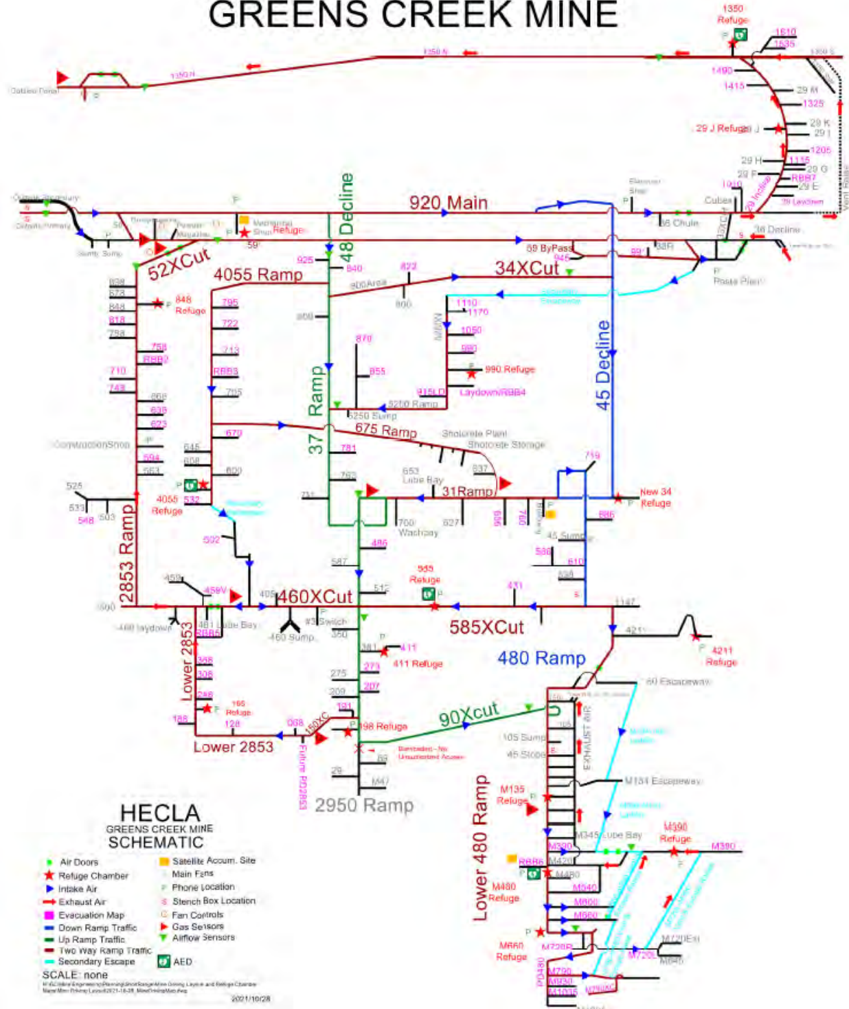
Figure 13-1: Underground Mine General Layout Schematic
