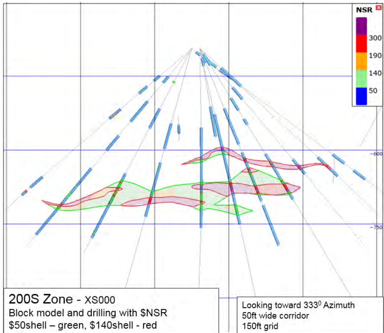
Figure 6-41: 200S Zone – Cross Section XS000
