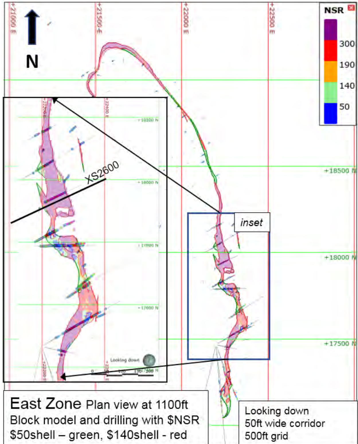
Figure 6-17: East Zone – Level Plan 1100
