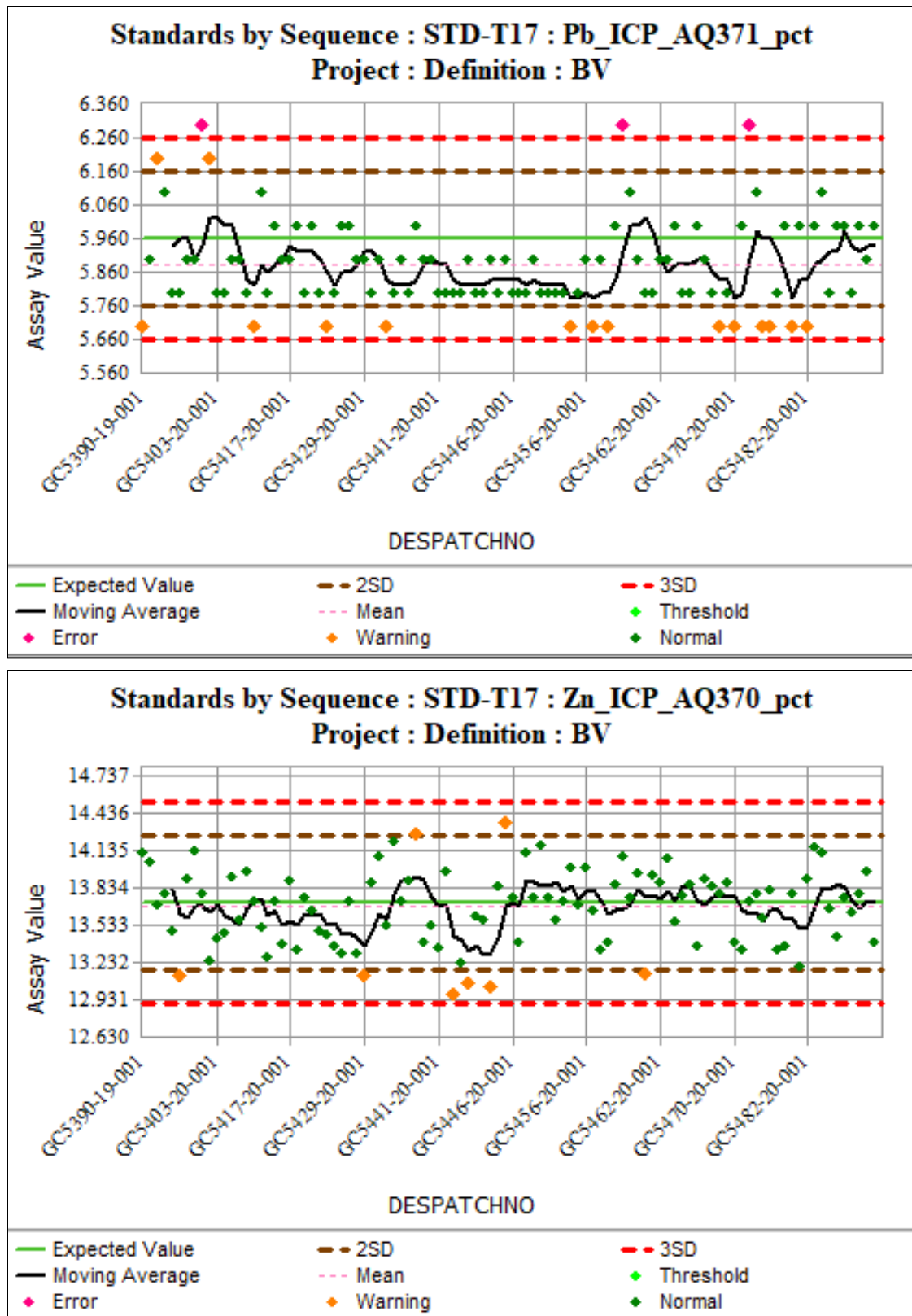
Figure 8-2: Standard Control Charts – Standard T17: Pb, Zn – Bureau Veritas 2020
