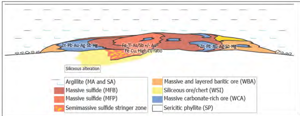
Figure 6-8: Simplified Mineralization Cross-Section
